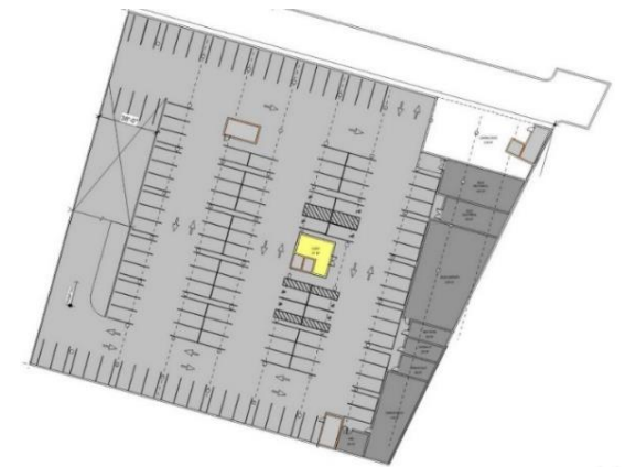
Basement Level 1 Plan Floor area – 57,780 SF
